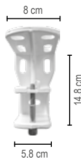
Mensola P/S 9000 IN Cover Max
